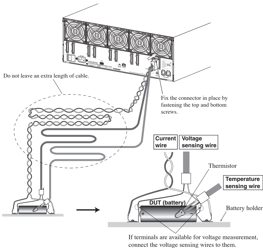
Fig. 2-5 Output Cable Connection
