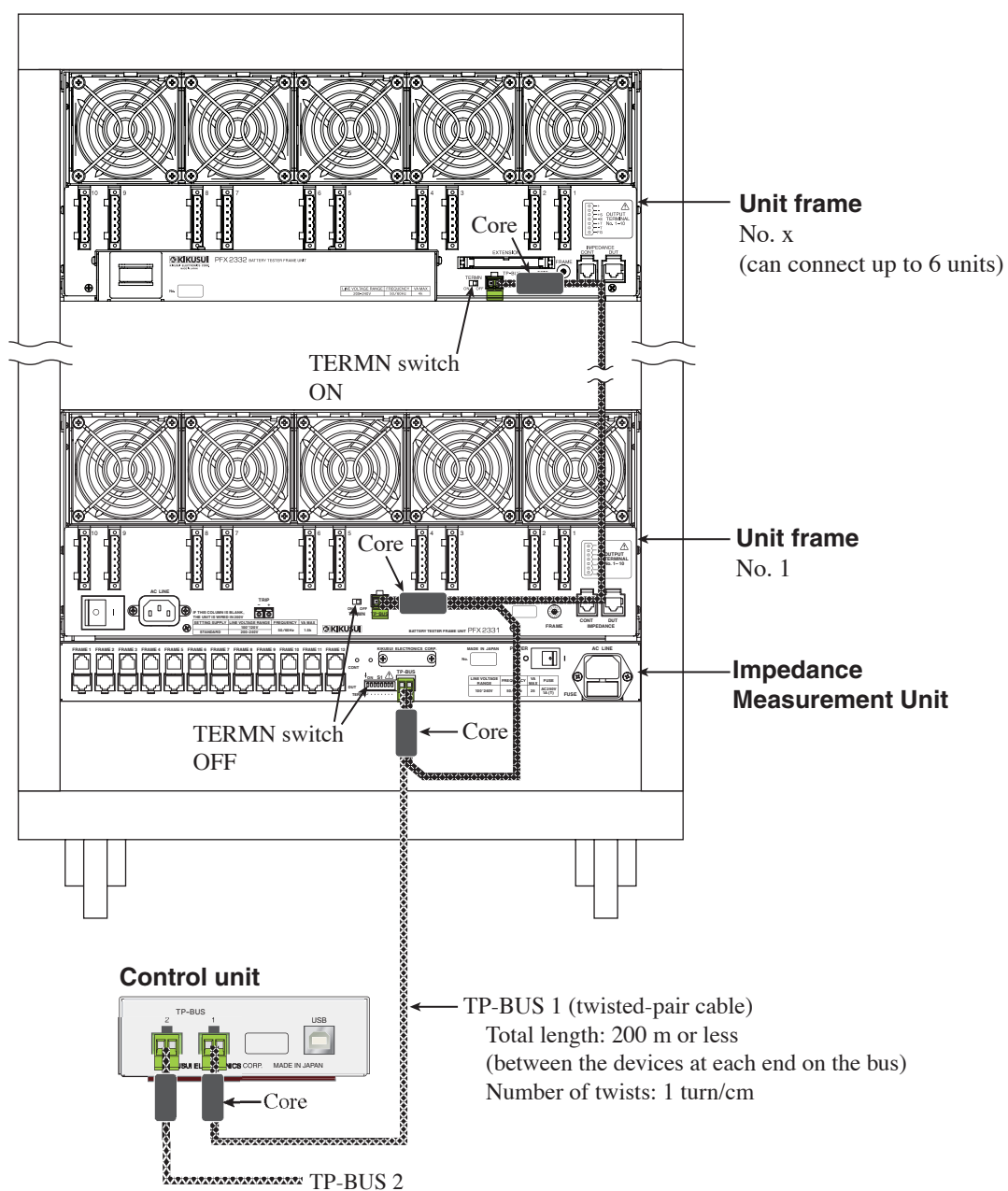
Fig. 1-11 TP-BUS Connection
