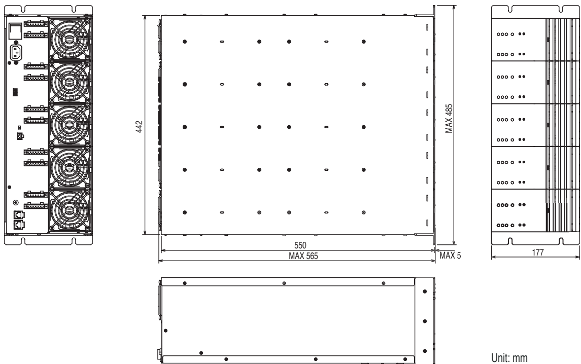
Fig.5-1 PFX2331 5-Unit Frame (The figure shows the case when PFX2011s are installed)
