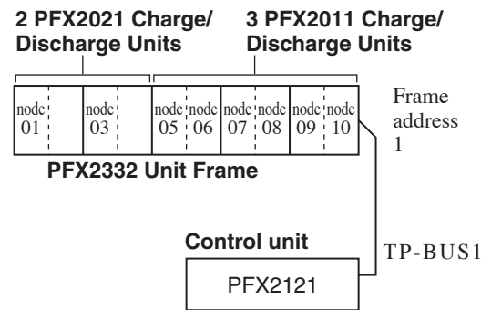
Fig. 1-10 Example When a Mixture of PFX2021s and PFX2011s Are Installed
