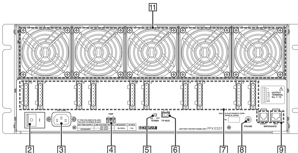
Fig. 3-2 PFX2331 Rear Panel
