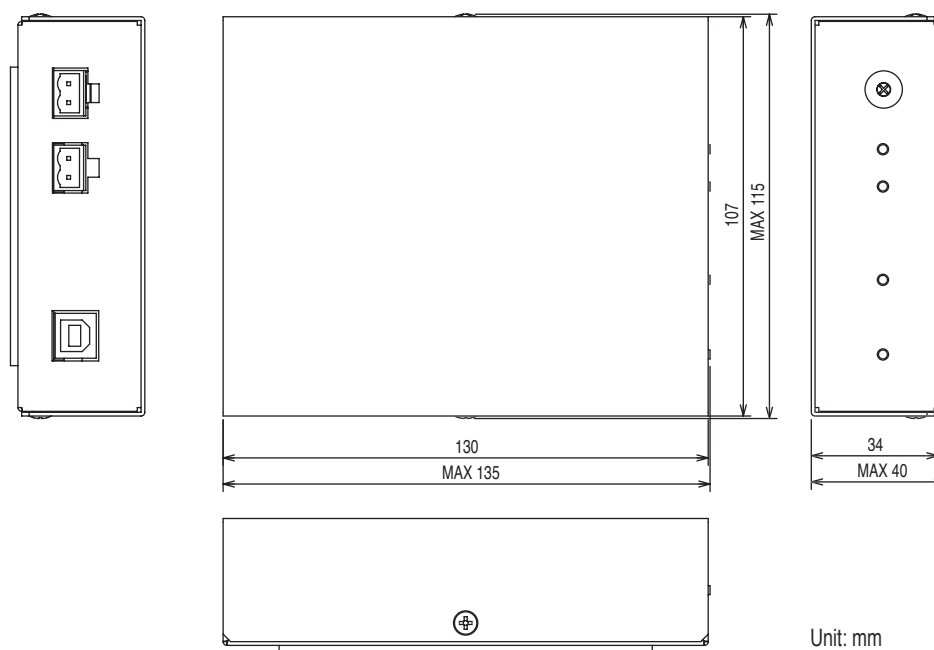
Fig. 5-3 PFX2121 120-ch Control Unit
