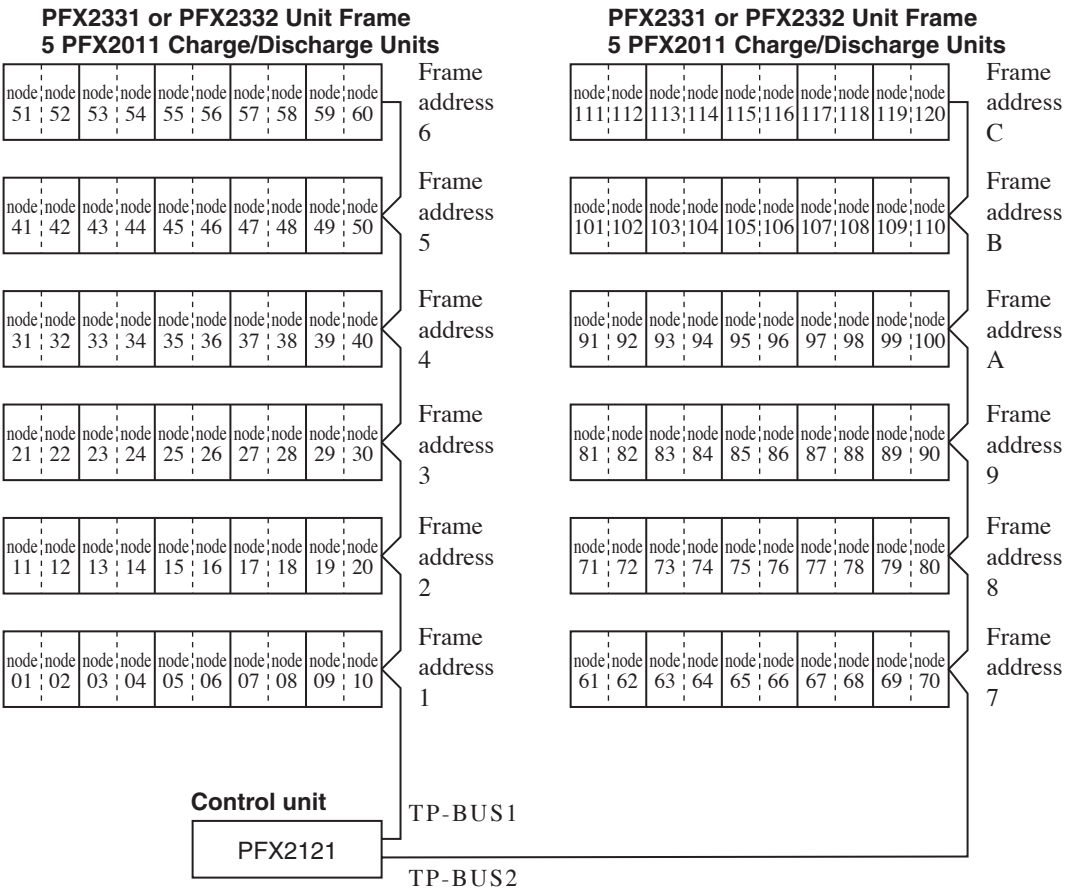
Fig. 1-8 Frame Addresses and Node Numbers (Example of 120-Channel Connection Using PFX2011s)
