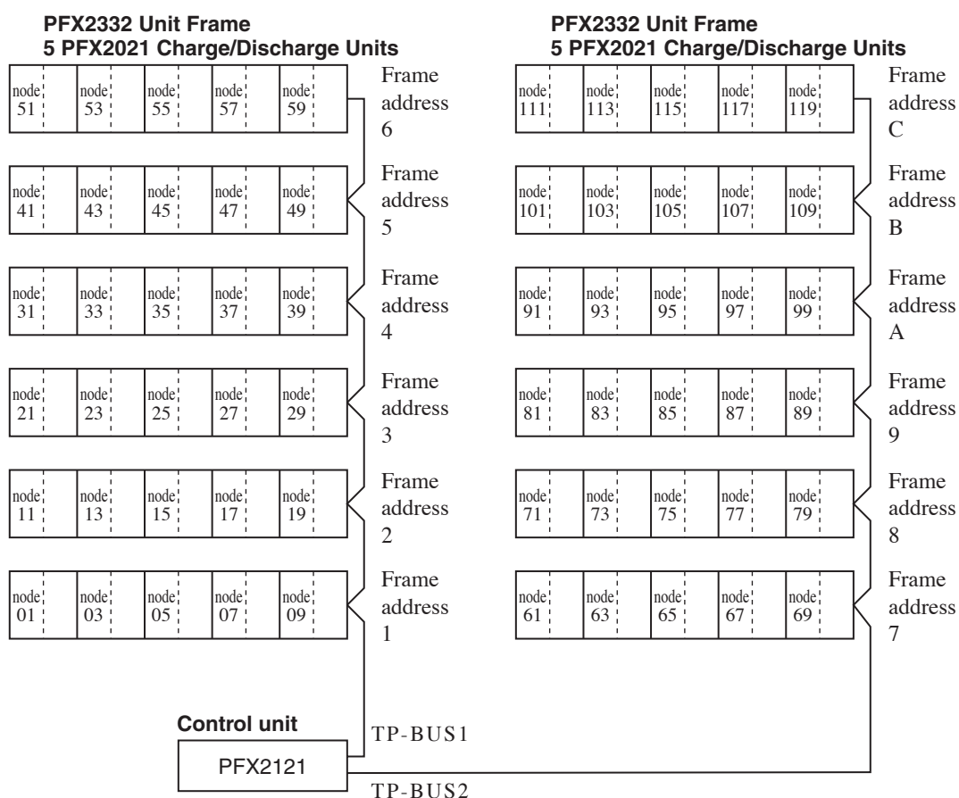
Fig. 1-9 Frame Addresses and Node Numbers (Example of 60-Channel Connection Using PFX2021s)
