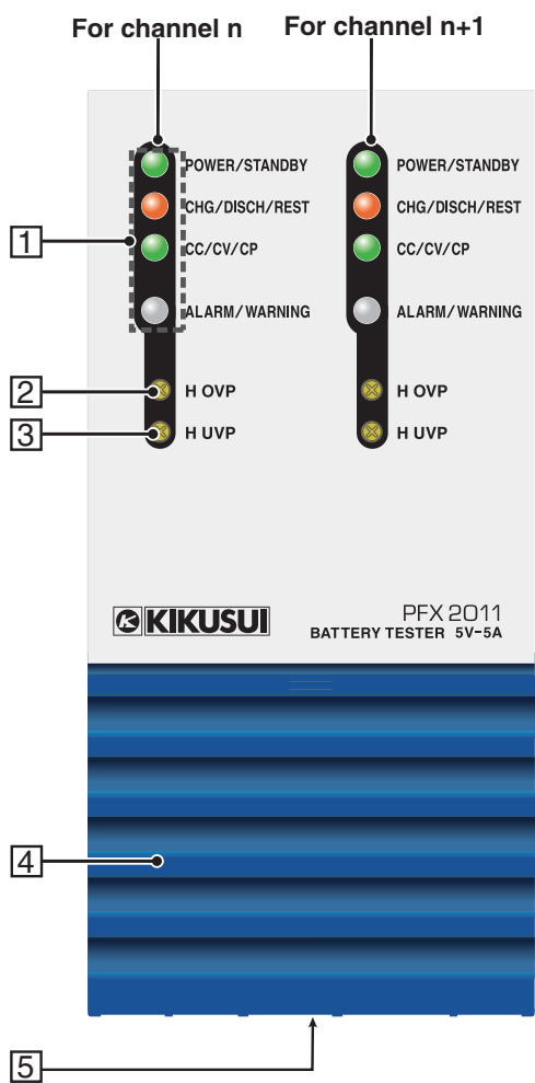
Fig. 3-4 PFX2011 Front Panel
