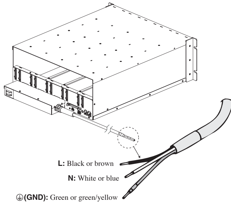
Fig. 1-3 Power cord of the PFX2332
