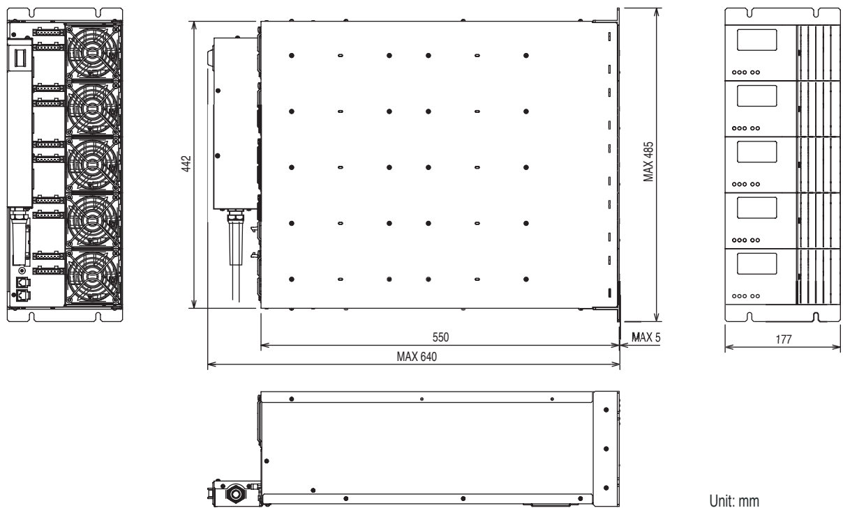
Fig. 5-2 PFX2332 Unit Frame (The figure shows the case when PFX2021s are installed)
