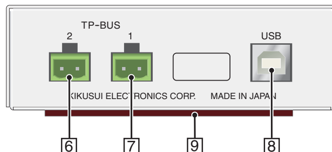
Fig. 3-7 Rear Panel of the PFX2121
