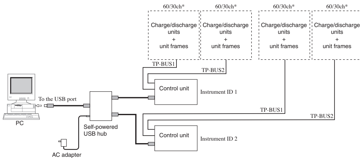
Fig. 1-17 Connection Example of Two Control Units
