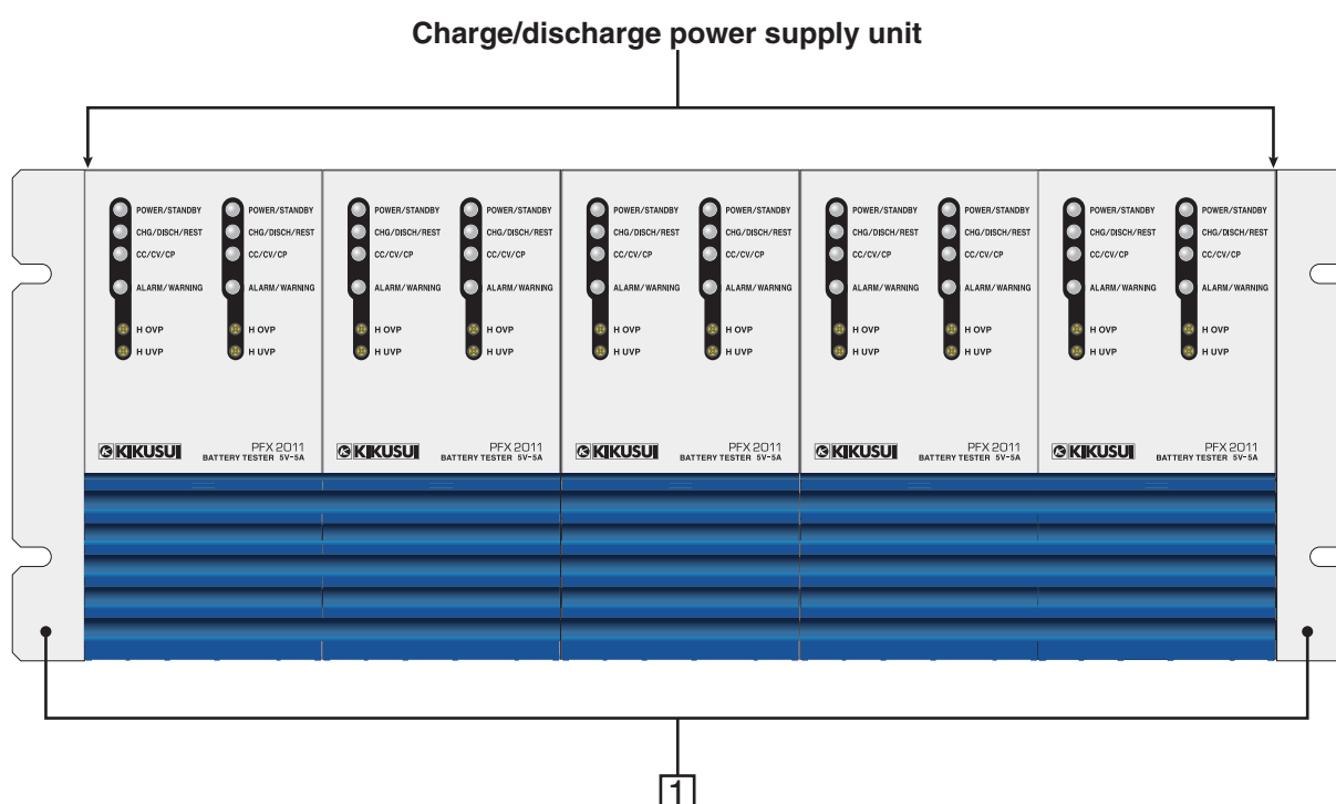
Fig.3-1 PFX2331 or PFX2332 Front Panel
