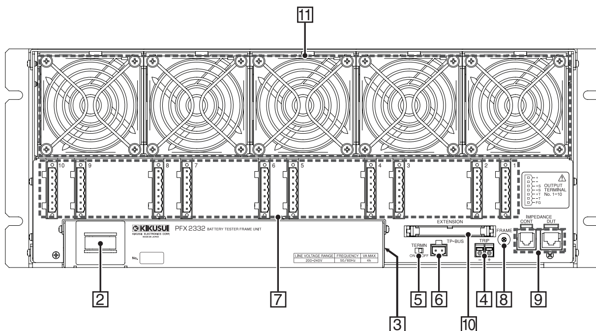
Fig. 3-3 PFX2332 Rear Panel
