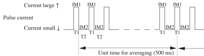
Fig. A-9 Averaging Example 1 of Pulse Current Measurement
