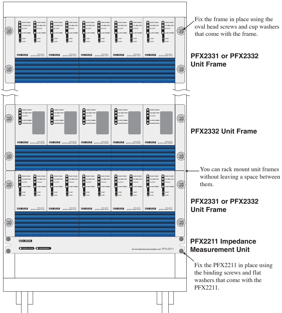
Fig. 1-1 Rack Mounting
